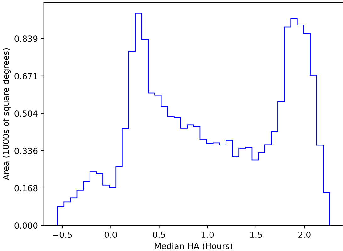
too_100_1v3.4_10yrs WFD all bands: Median HA
