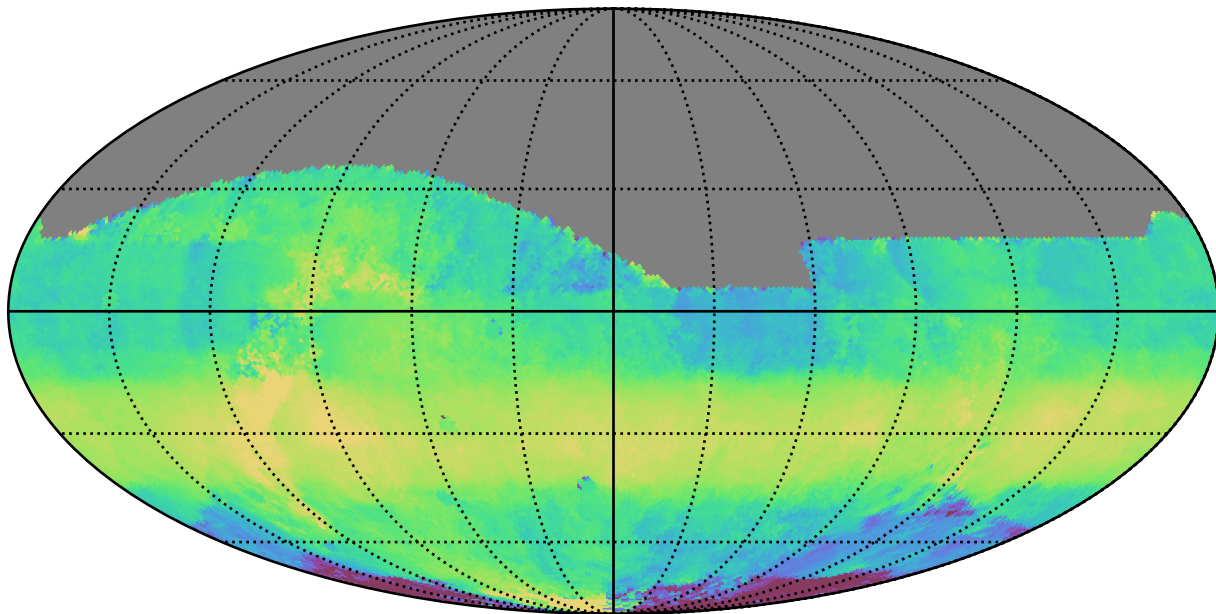
too_100_1v3.4_10yrs All sky z band: Median HA
