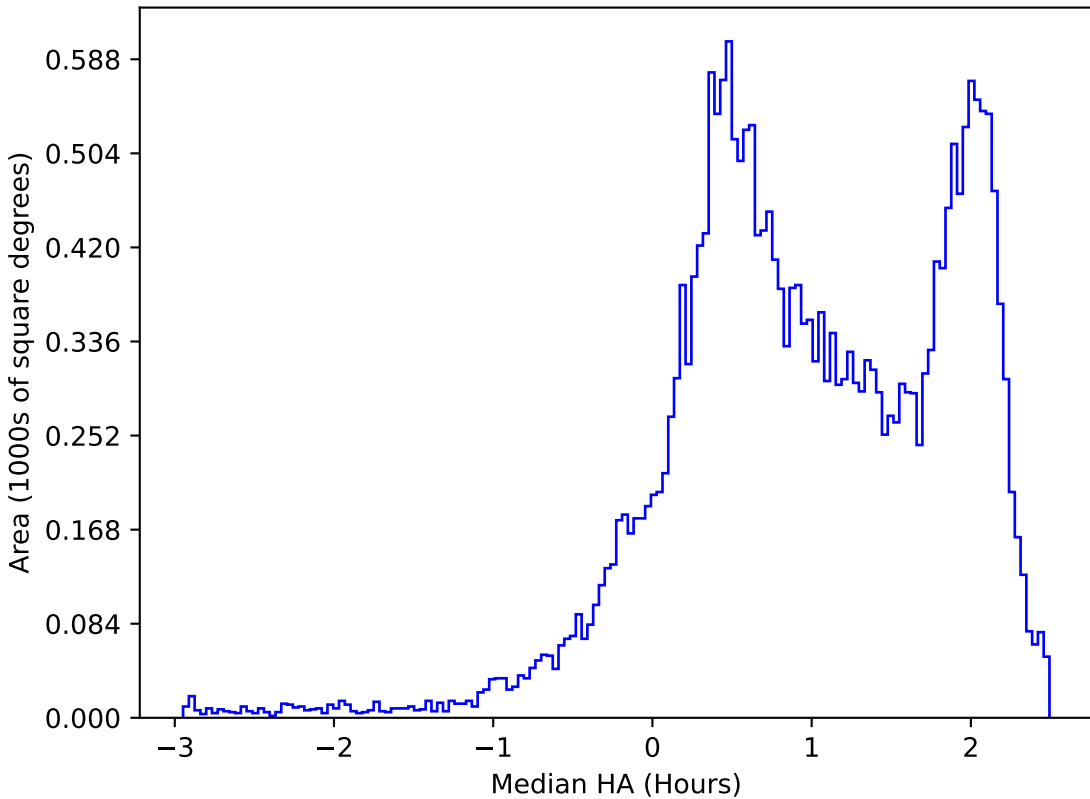
too_100_1v3.4_10yrs All sky z band: Median HA
