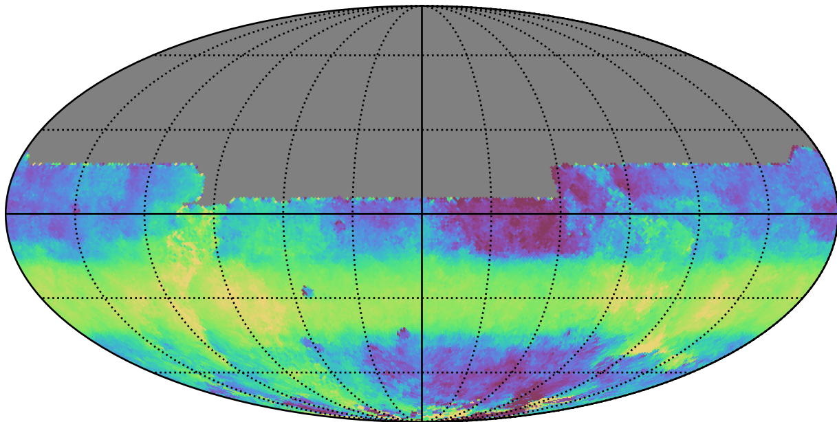
too_100_1v3.4_10yrs All sky y band: Median HA
