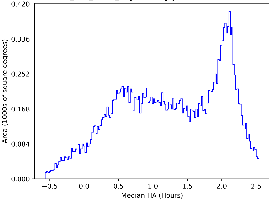
too_100_1v3.4_10yrs All sky y band: Median HA
