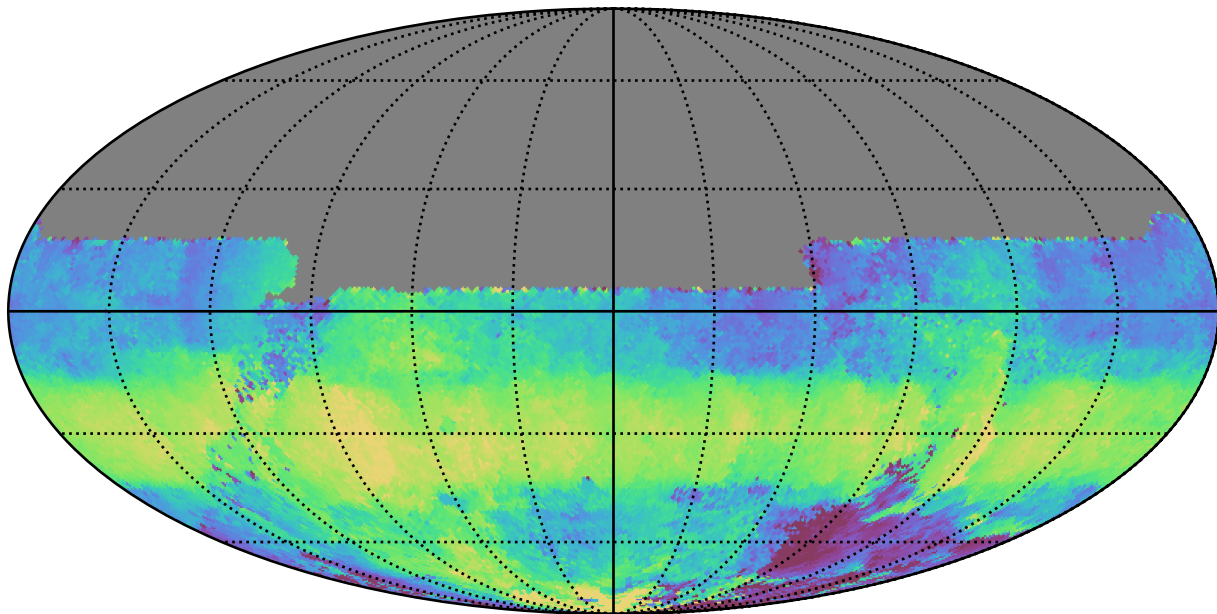
too_100_1v3.4_10yrs All sky u band: Median HA
