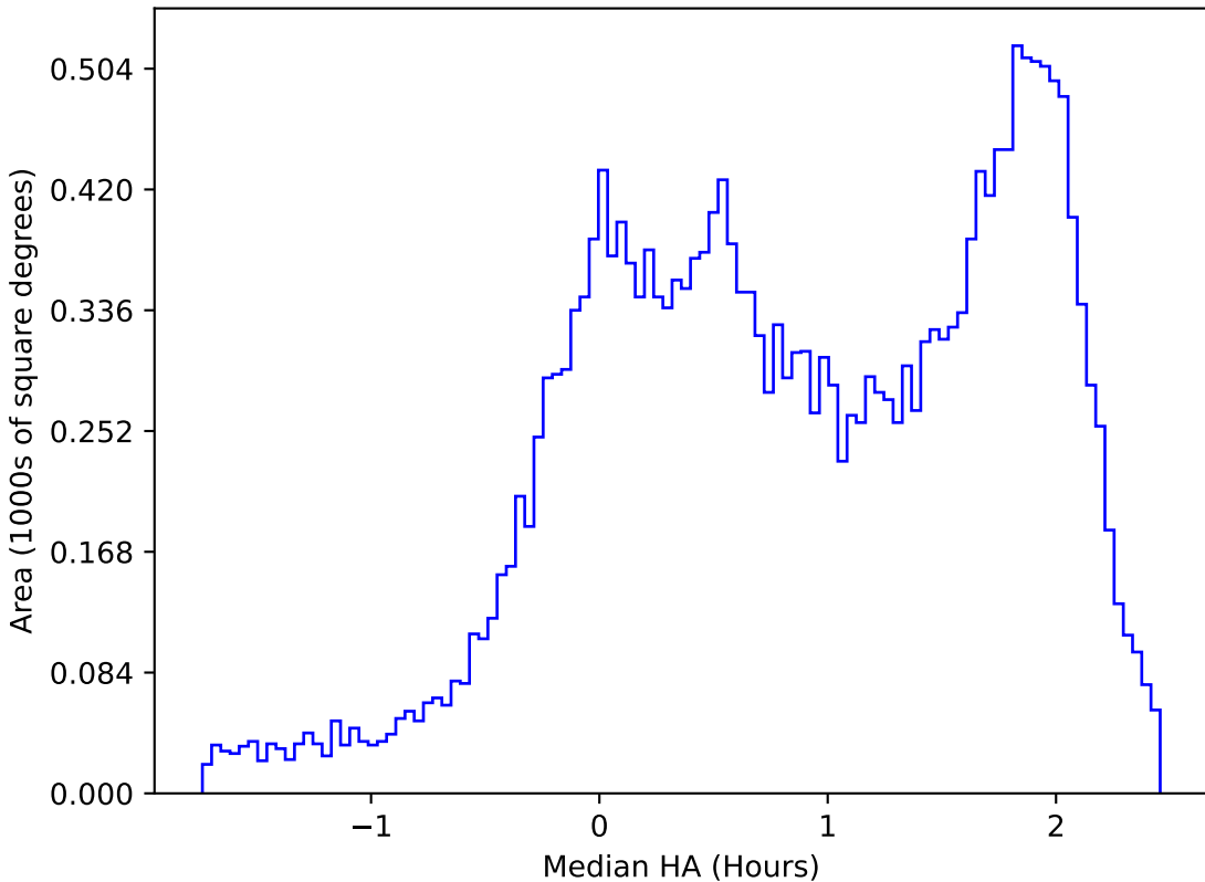
too_100_1v3.4_10yrs All sky u band: Median HA
