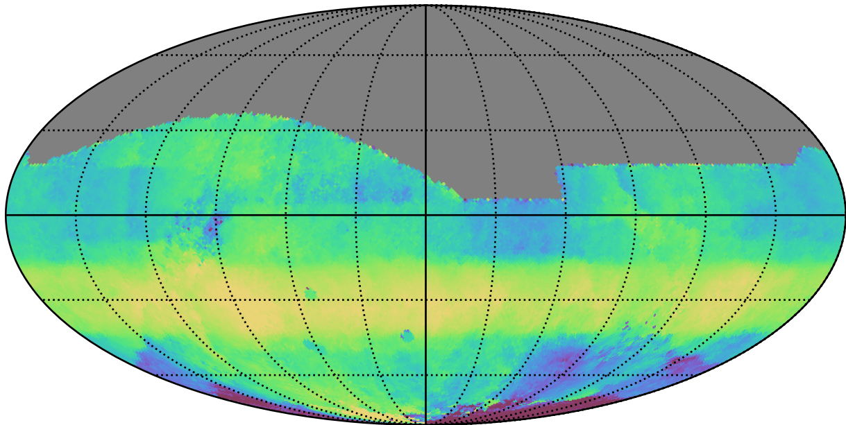
too_100_1v3.4_10yrs All sky r band: Median HA
