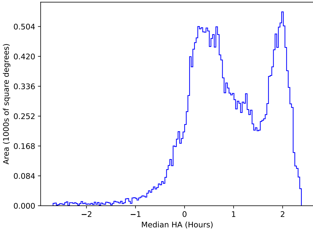
too_100_1v3.4_10yrs All sky i band: Median HA
