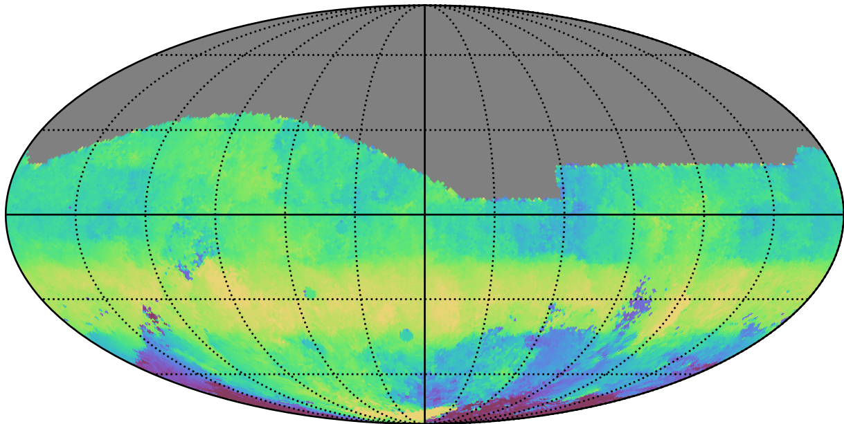
too_100_1v3.4_10yrs All sky g band: Median HA
