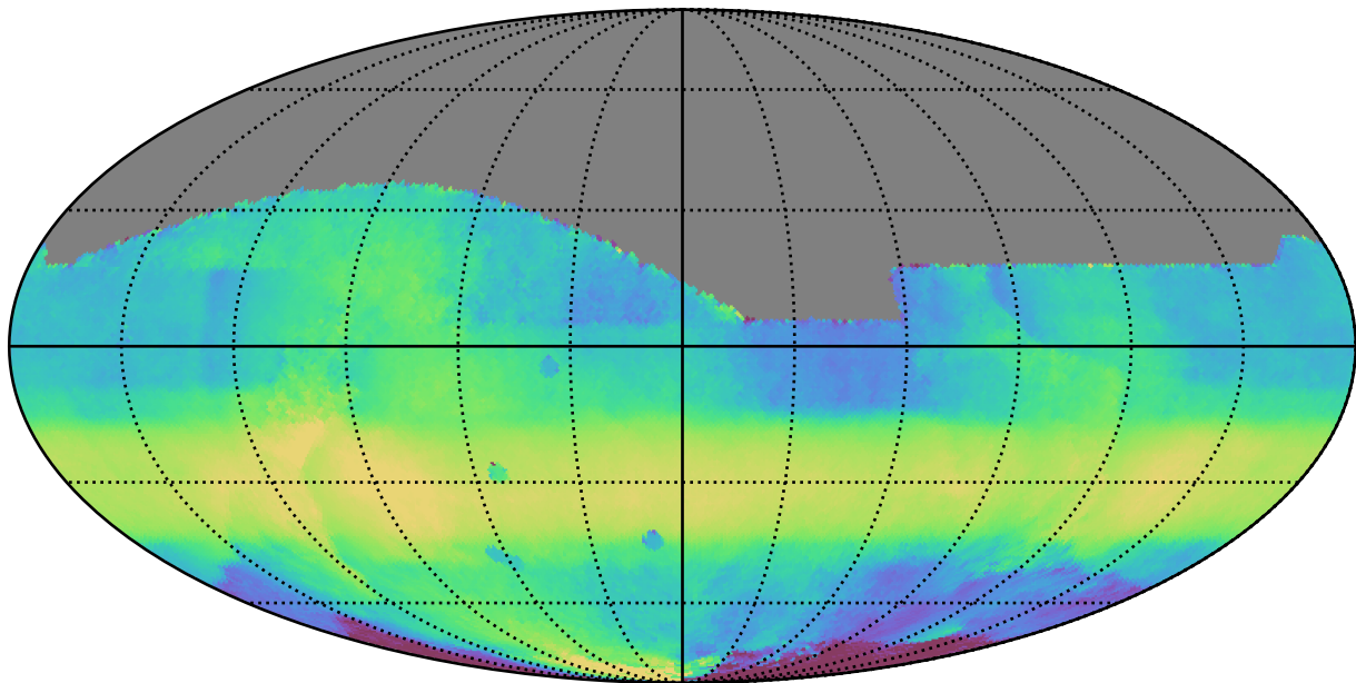
too_100_1v3.4_10yrs All sky all bands: Median HA
