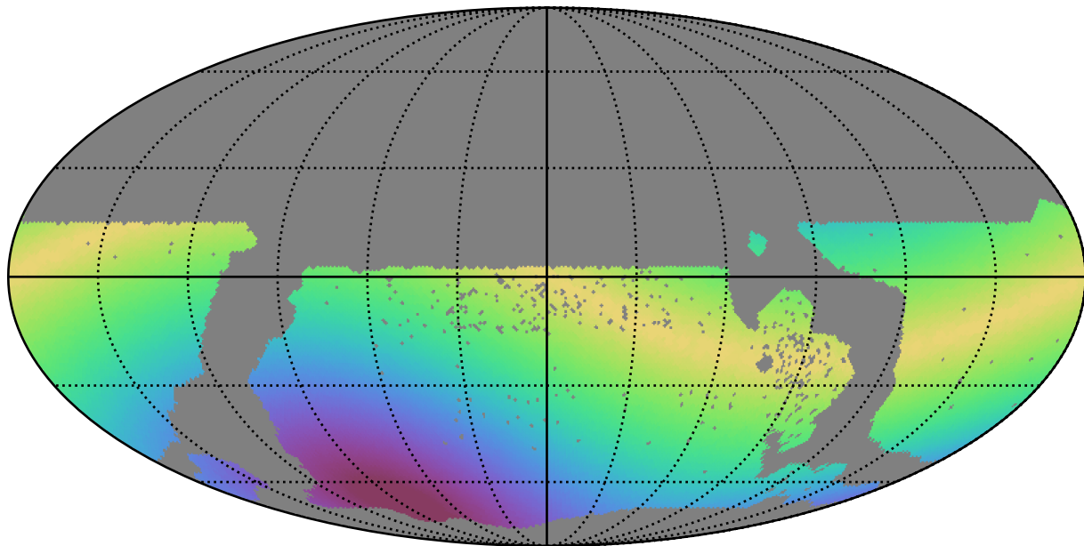
too_100_1v3.4_10yrs WFD z band: Max solarElong
