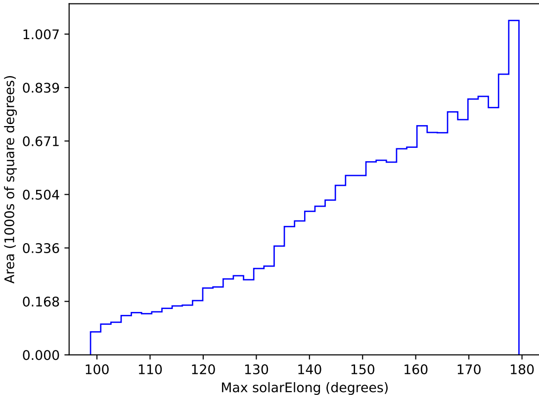
too_100_1v3.4_10yrs WFD z band: Max solarElong
