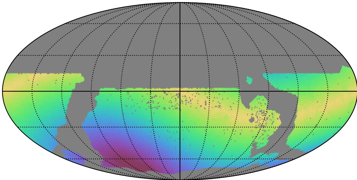
too_100_1v3.4_10yrs WFD u band: Max solarElong
