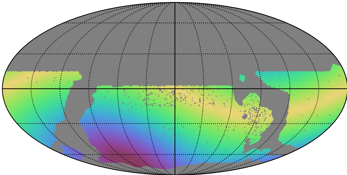
too_100_1v3.4_10yrs WFD r band: Max solarElong
