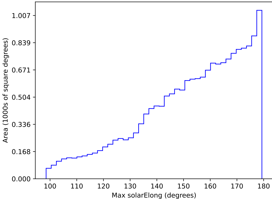
too_100_1v3.4_10yrs WFD r band: Max solarElong
