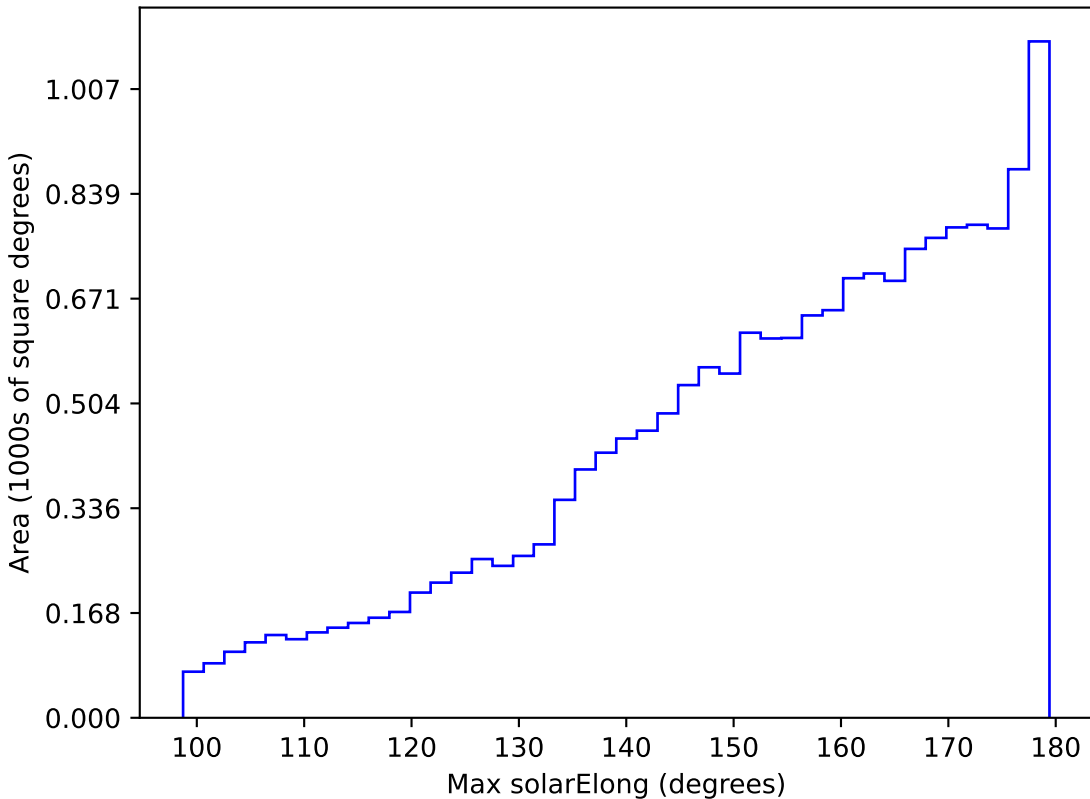
too_100_1v3.4_10yrs WFD i band: Max solarElong
