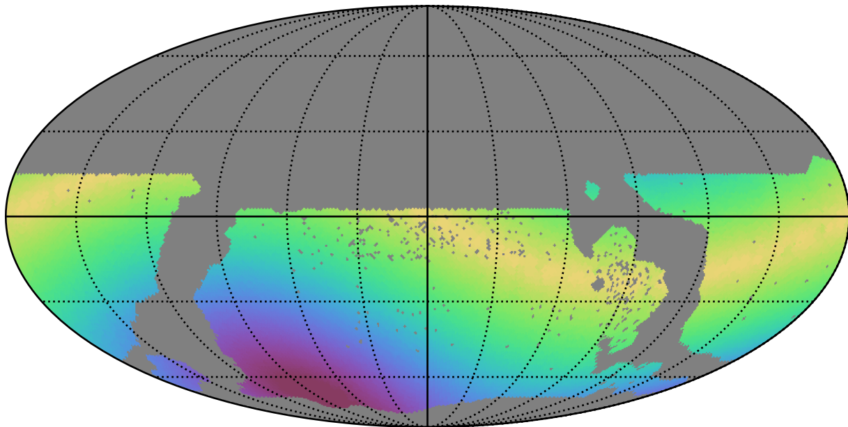
too_100_1v3.4_10yrs WFD g band: Max solarElong
