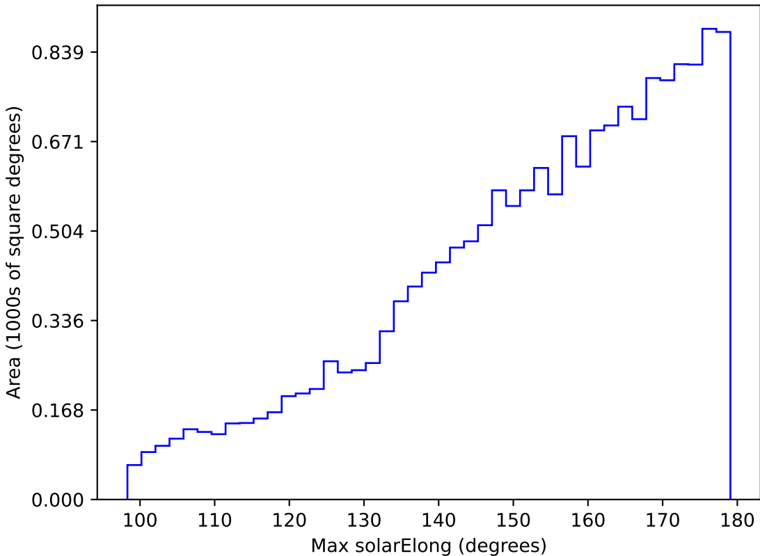
too_100_1v3.4_10yrs WFD g band: Max solarElong
