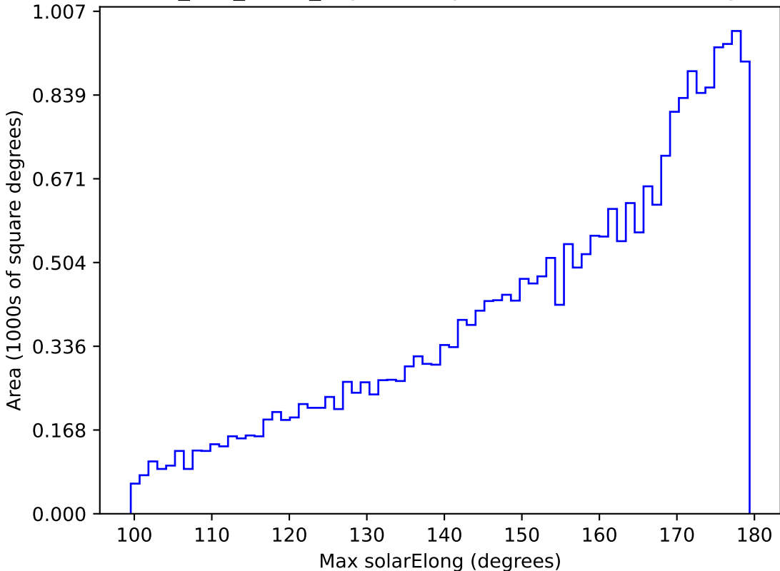
too_100_1v3.4_10yrs All sky z band: Max solarElong
