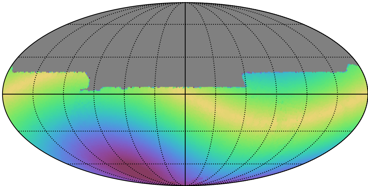
too_100_1v3.4_10yrs All sky y band: Max solarElong
