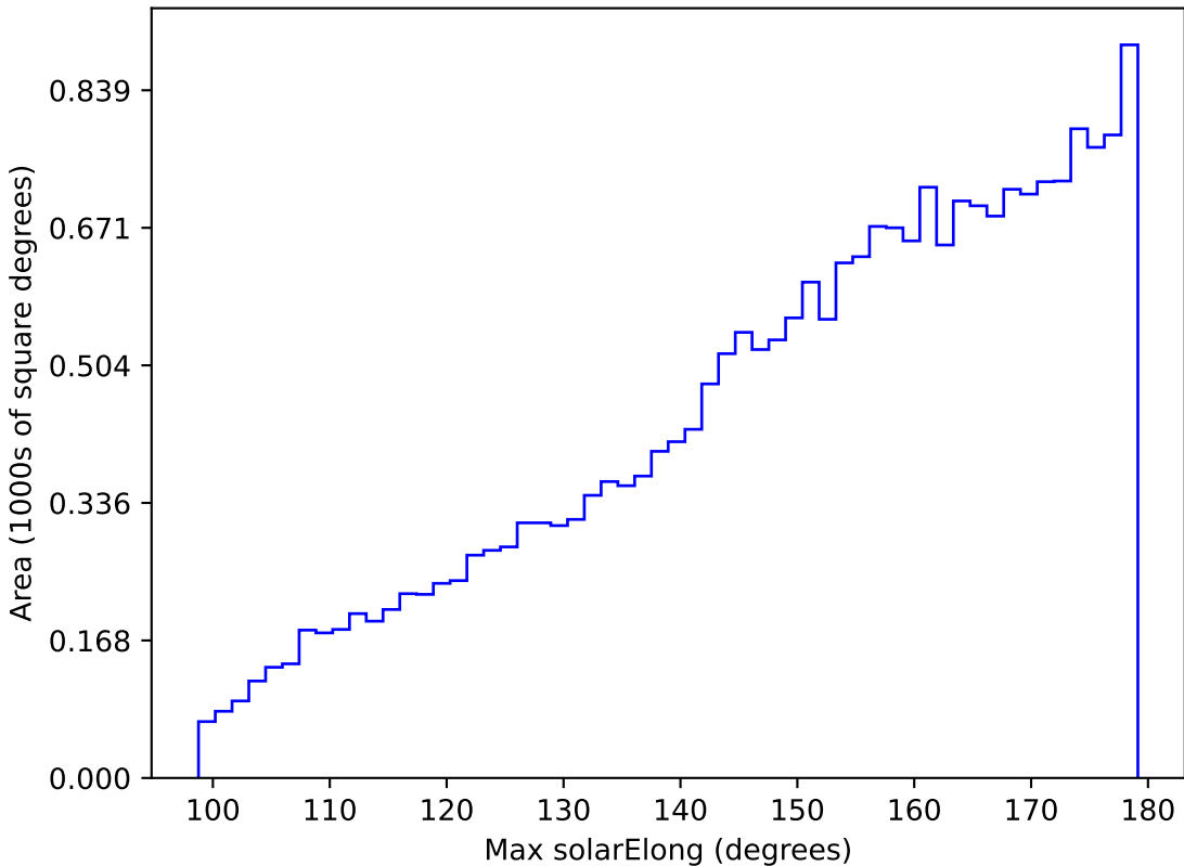
too_100_1v3.4_10yrs All sky y band: Max solarElong
