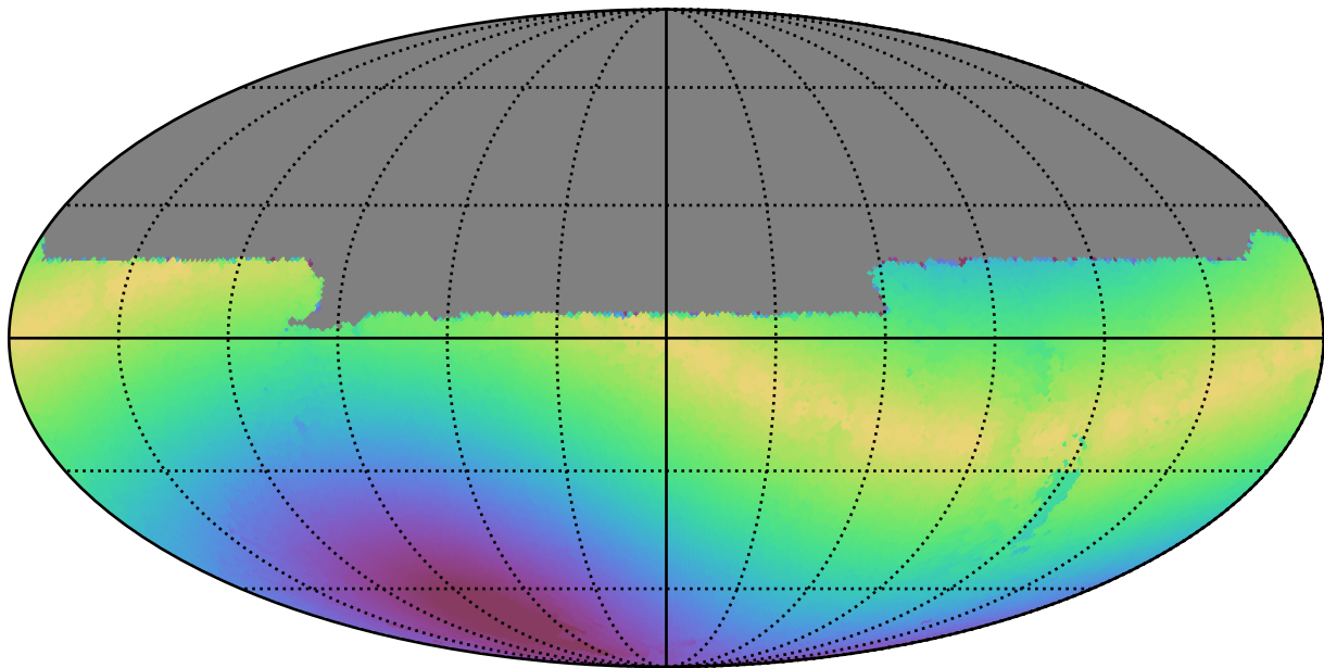
too_100_1v3.4_10yrs All sky u band: Max solarElong
