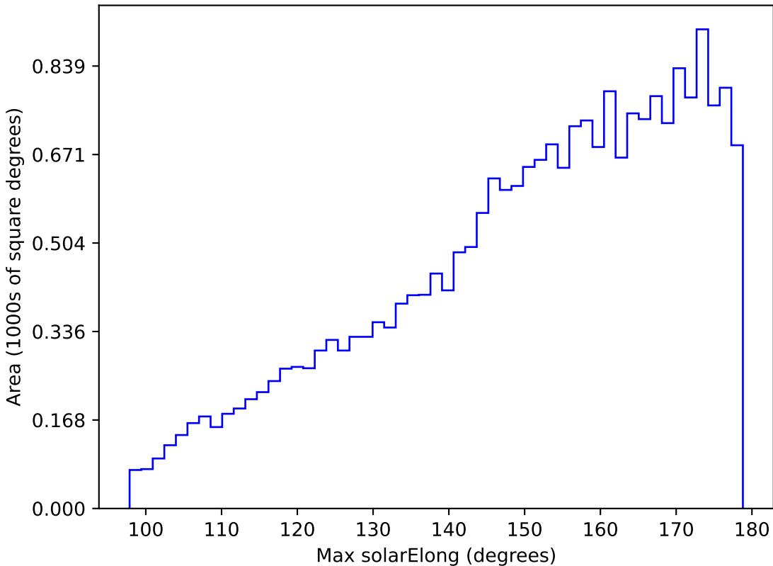
too_100_1v3.4_10yrs All sky u band: Max solarElong
