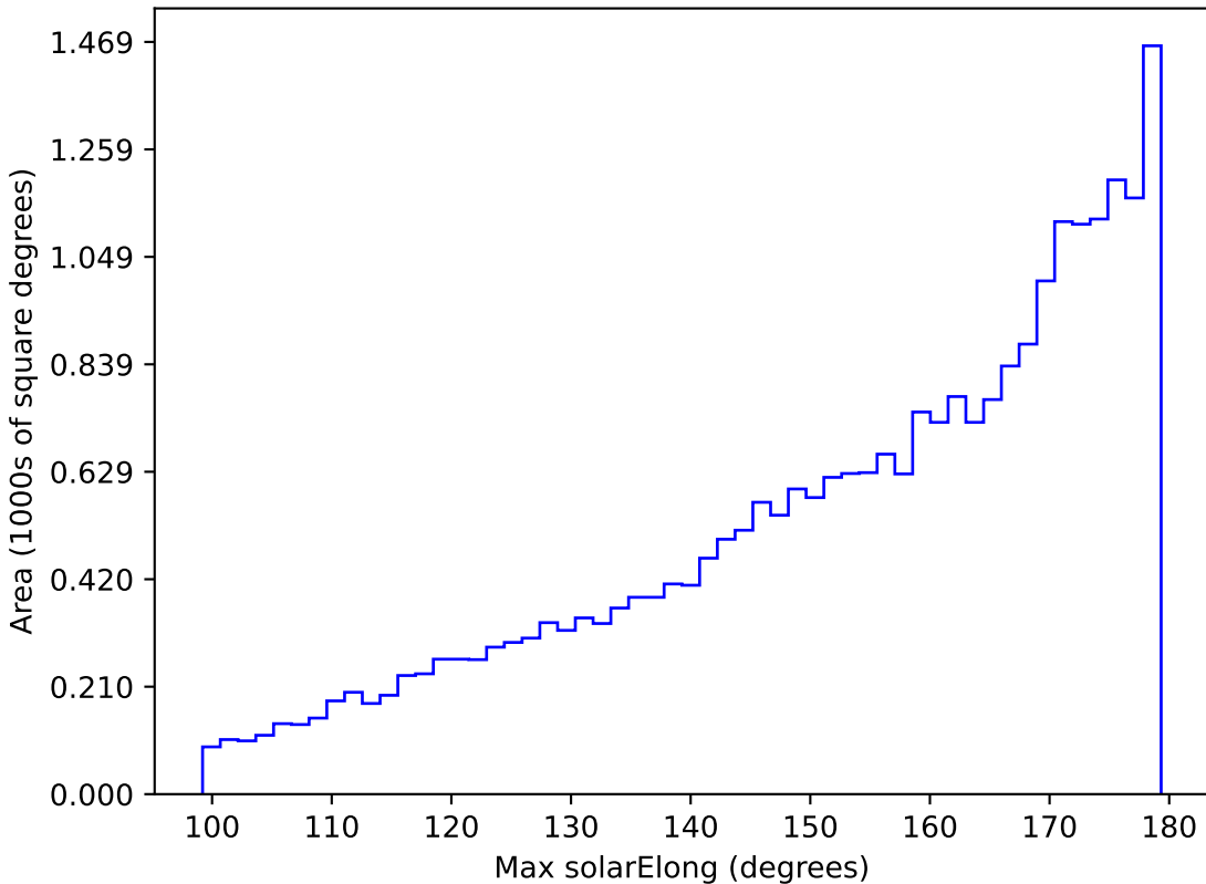
too_100_1v3.4_10yrs All sky r band: Max solarElong
