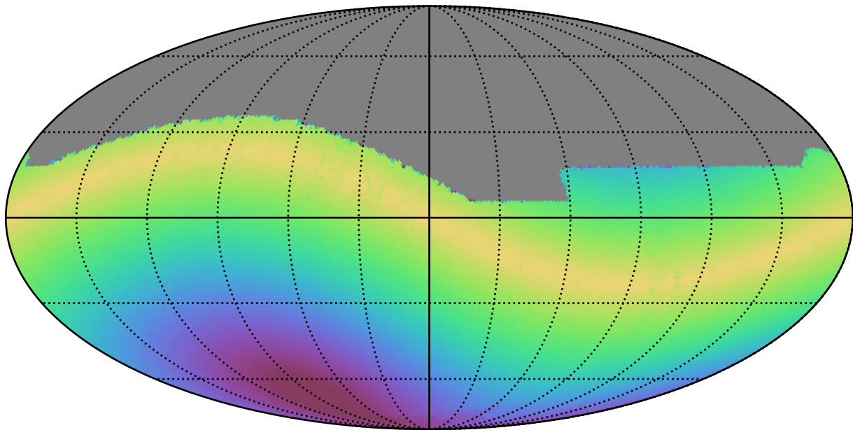
too_100_1v3.4_10yrs All sky i band: Max solarElong
