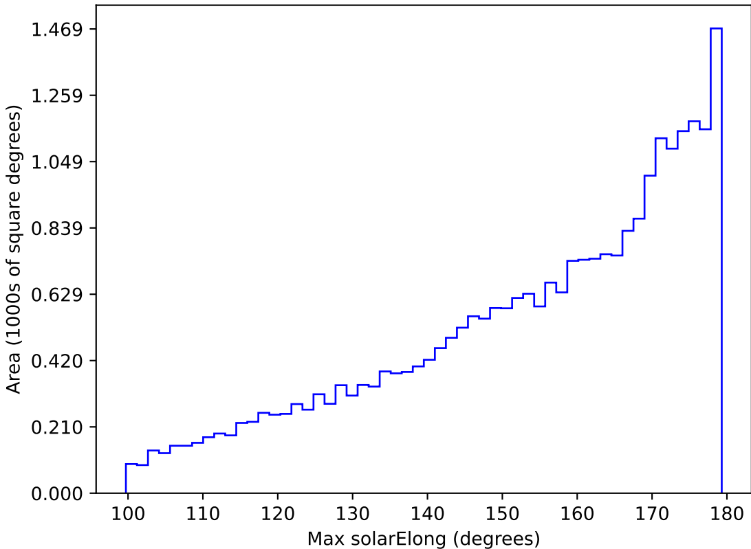
too_100_1v3.4_10yrs All sky i band: Max solarElong
