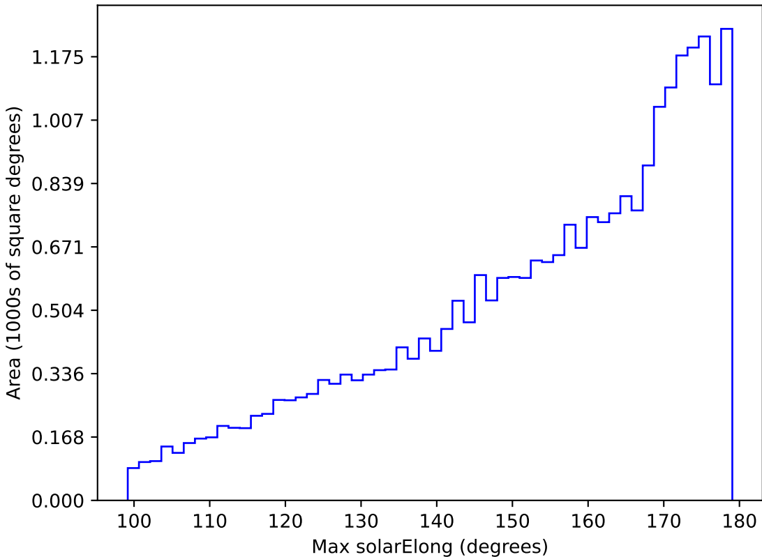
too_100_1v3.4_10yrs All sky g band: Max solarElong
