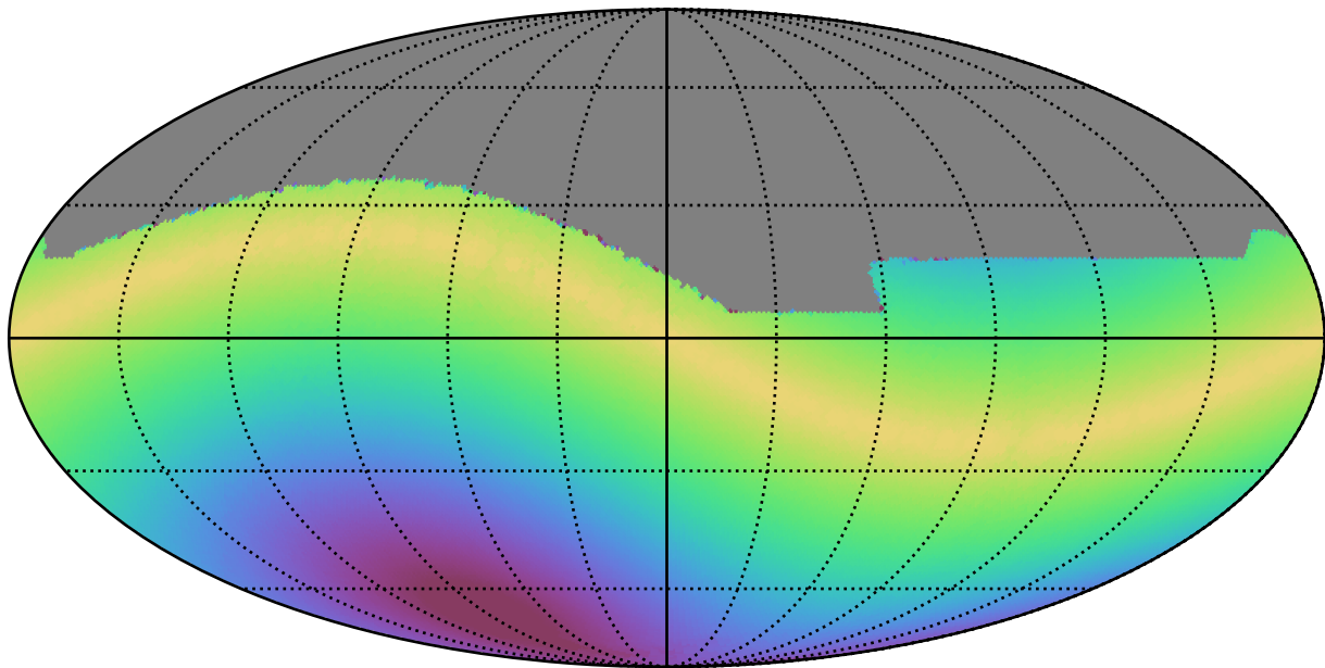
too_100_1v3.4_10yrs All sky all bands: Max solarElong
