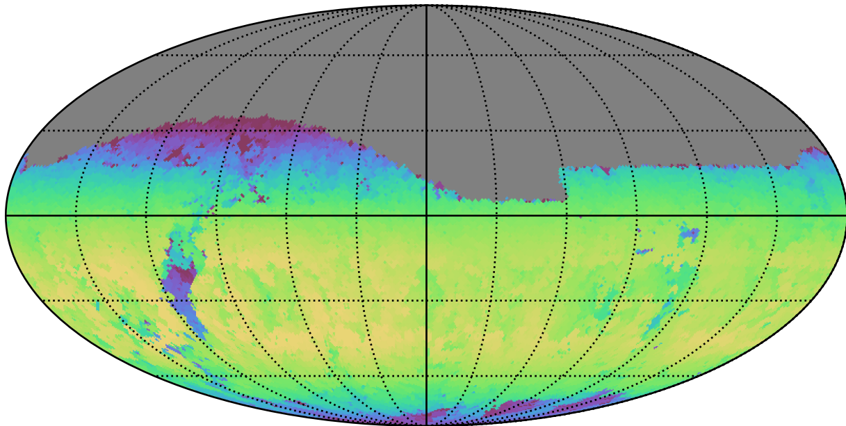
too_100_1v3.4_10yrs Yr 1 z band: Max skyBrightness
