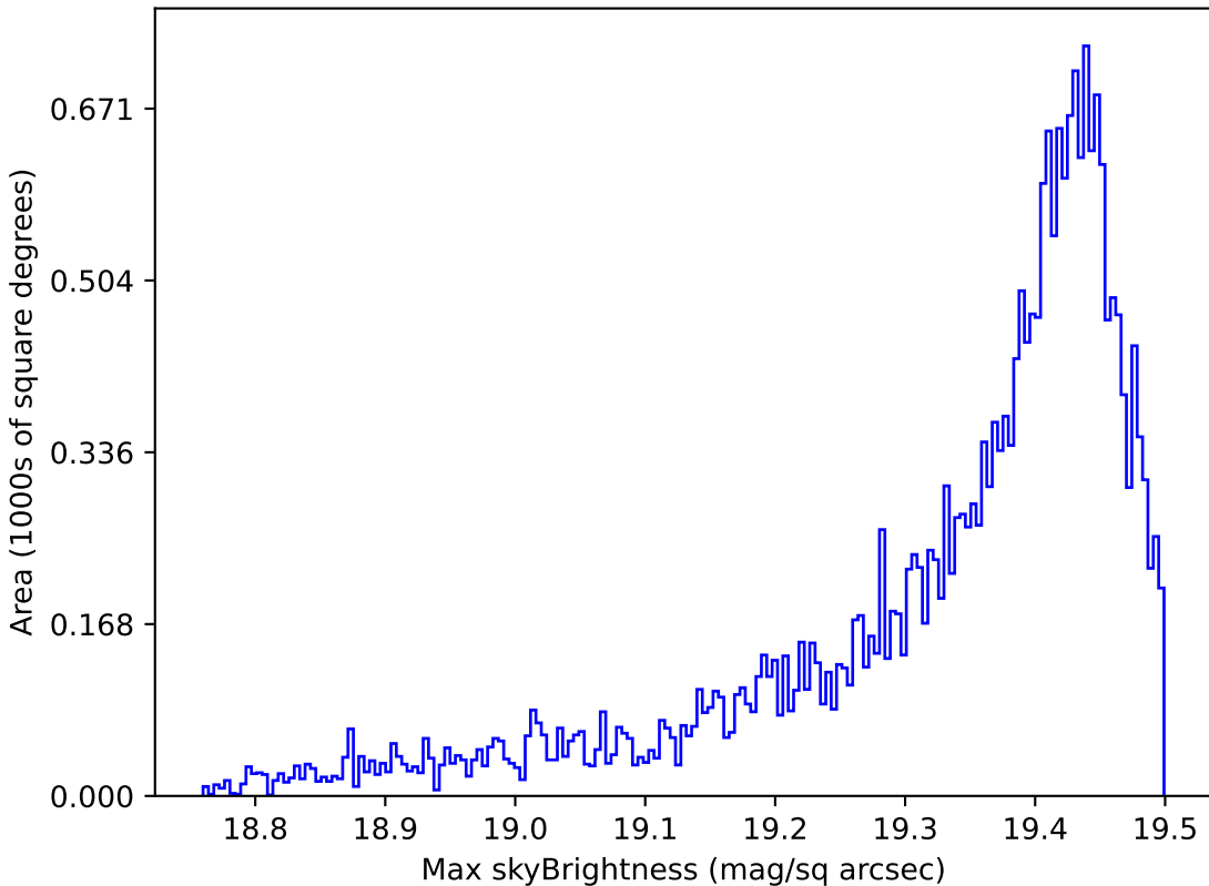
too_100_1v3.4_10yrs Yr 1 z band: Max skyBrightness
