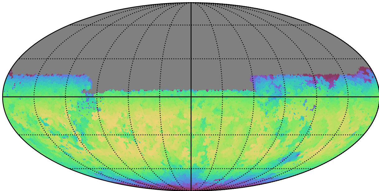
too_100_1v3.4_10yrs Yr 1 y band: Max skyBrightness
