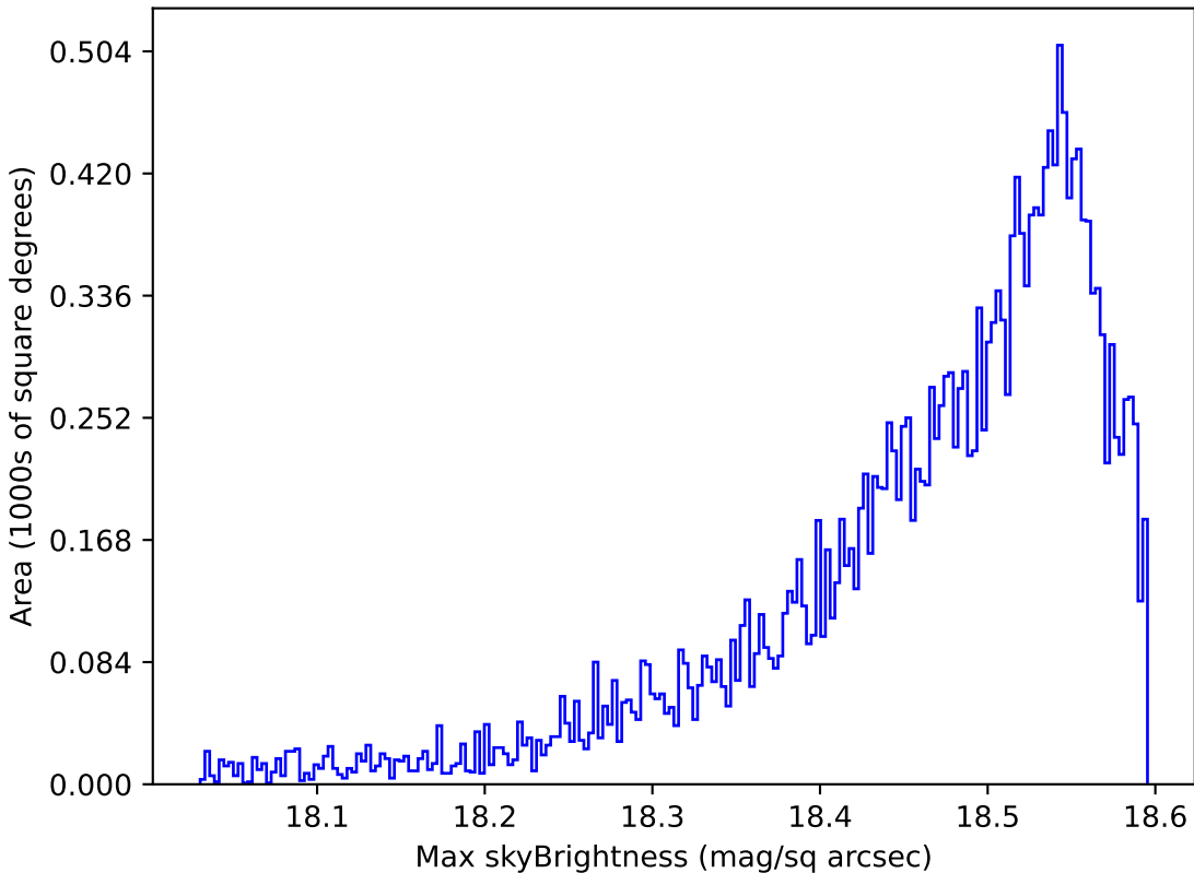
too_100_1v3.4_10yrs Yr 1 y band: Max skyBrightness
