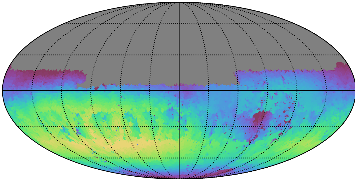
too_100_1v3.4_10yrs Yr 1 u band: Max skyBrightness
