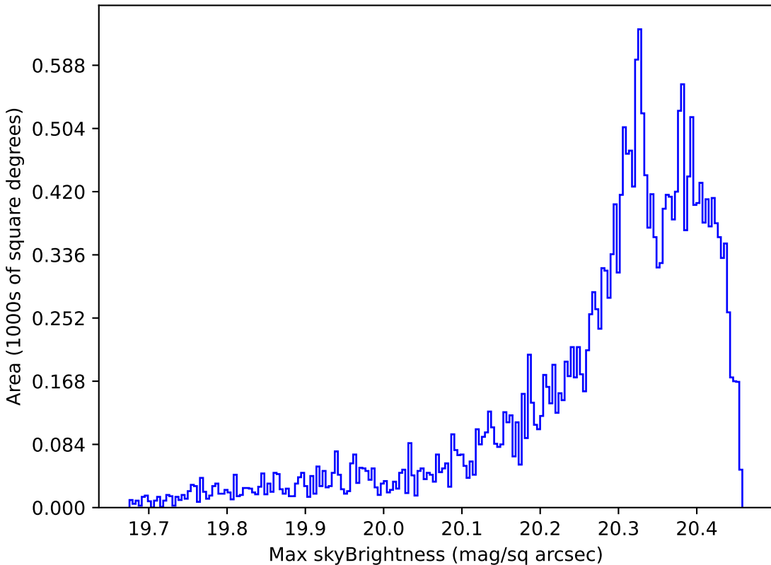
too_100_1v3.4_10yrs Yr 1 i band: Max skyBrightness
