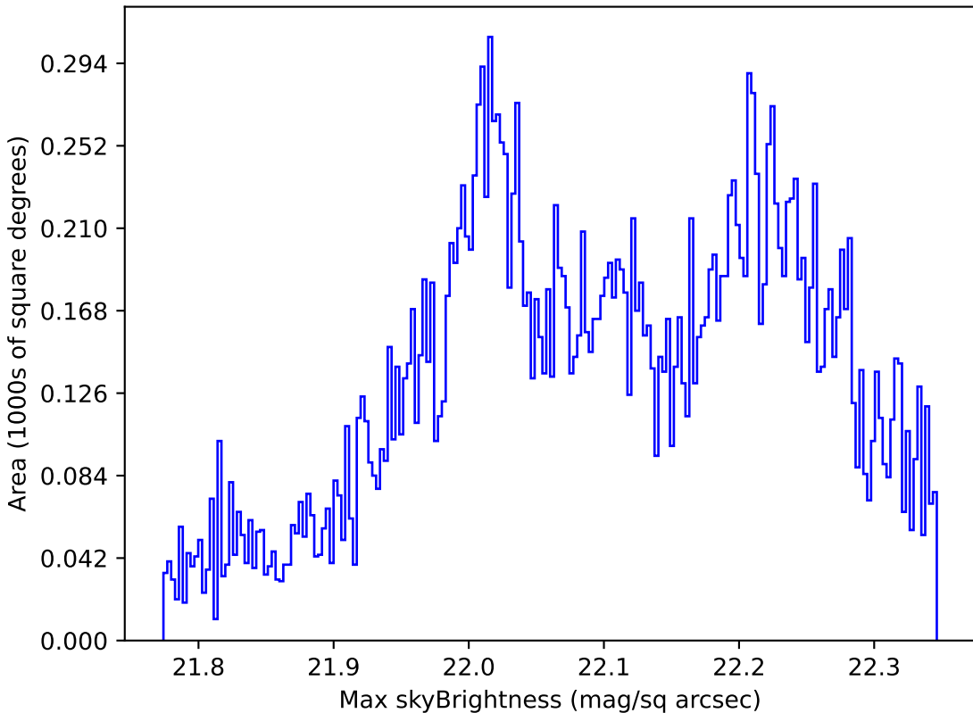
too_100_1v3.4_10yrs Yr 1 g band: Max skyBrightness
