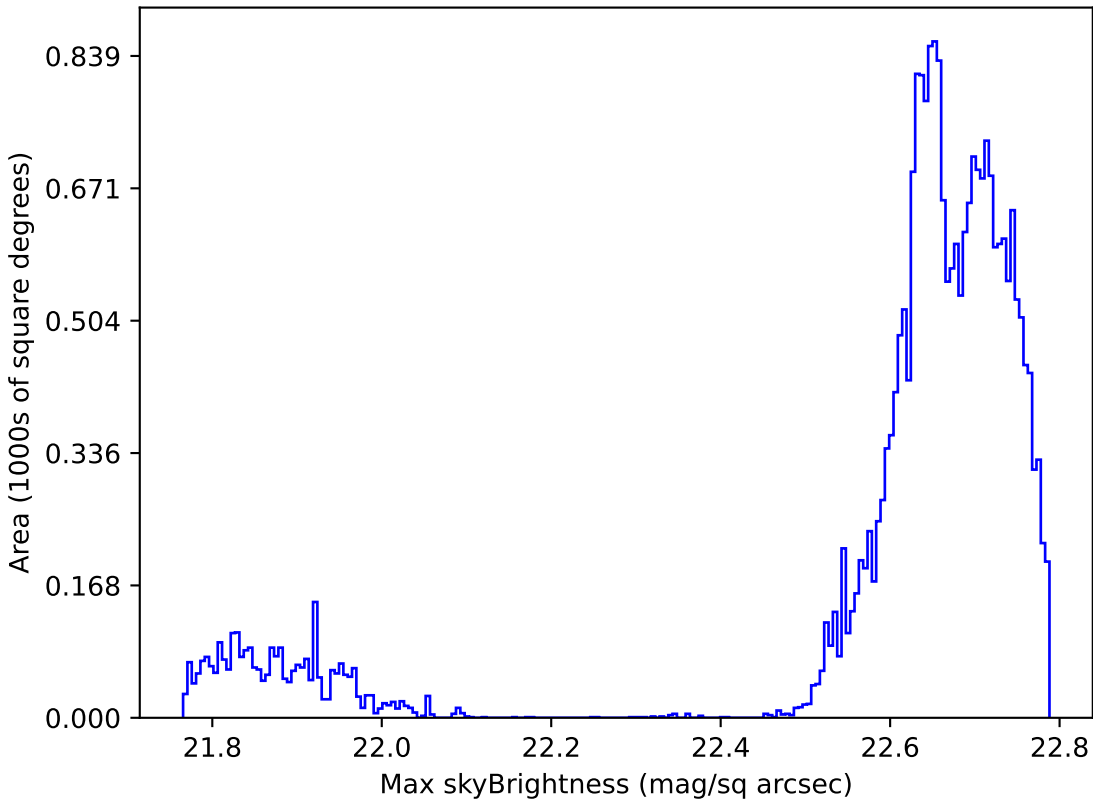
too_100_1v3.4_10yrs Yr 1 all bands: Max skyBrightness
