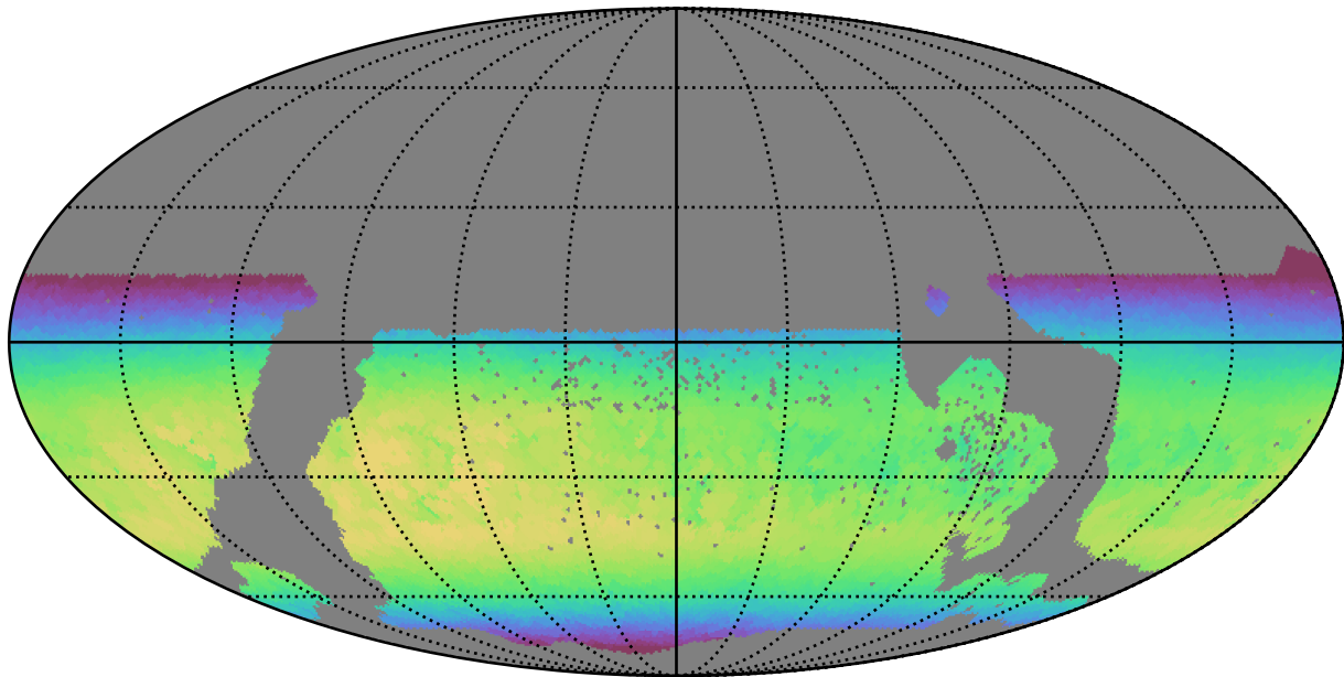
too_100_1v3.4_10yrs WFD z band: Max skyBrightness
