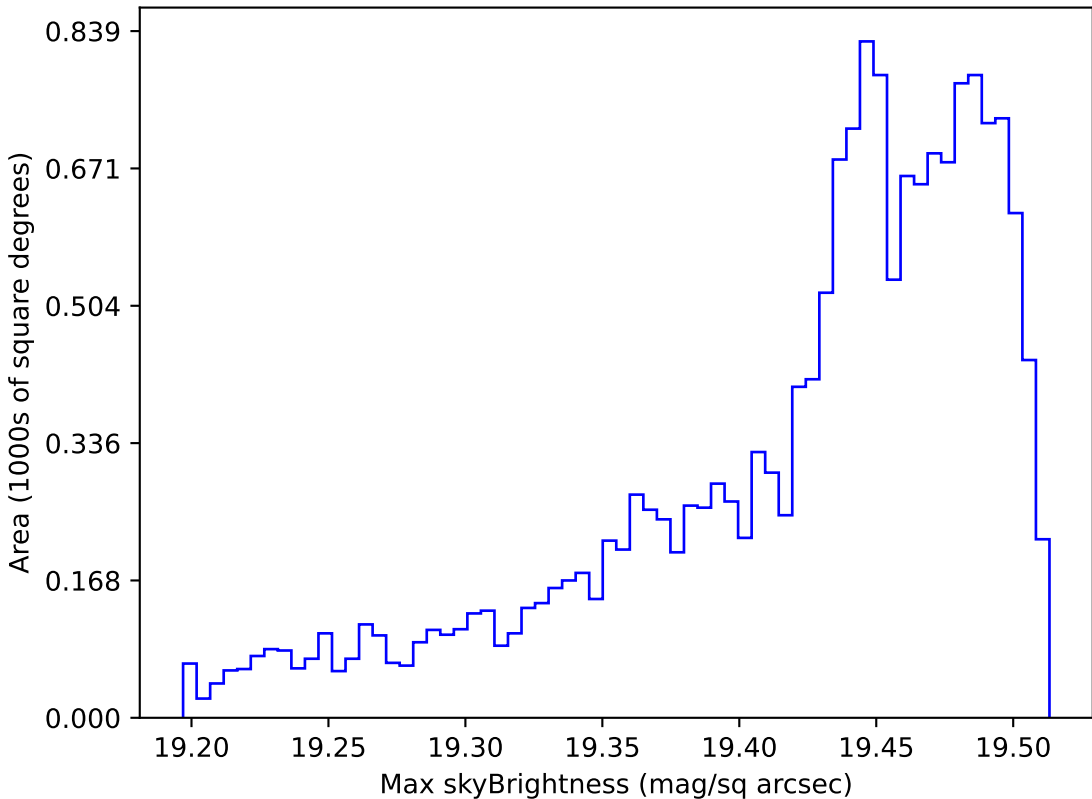
too_100_1v3.4_10yrs WFD z band: Max skyBrightness
