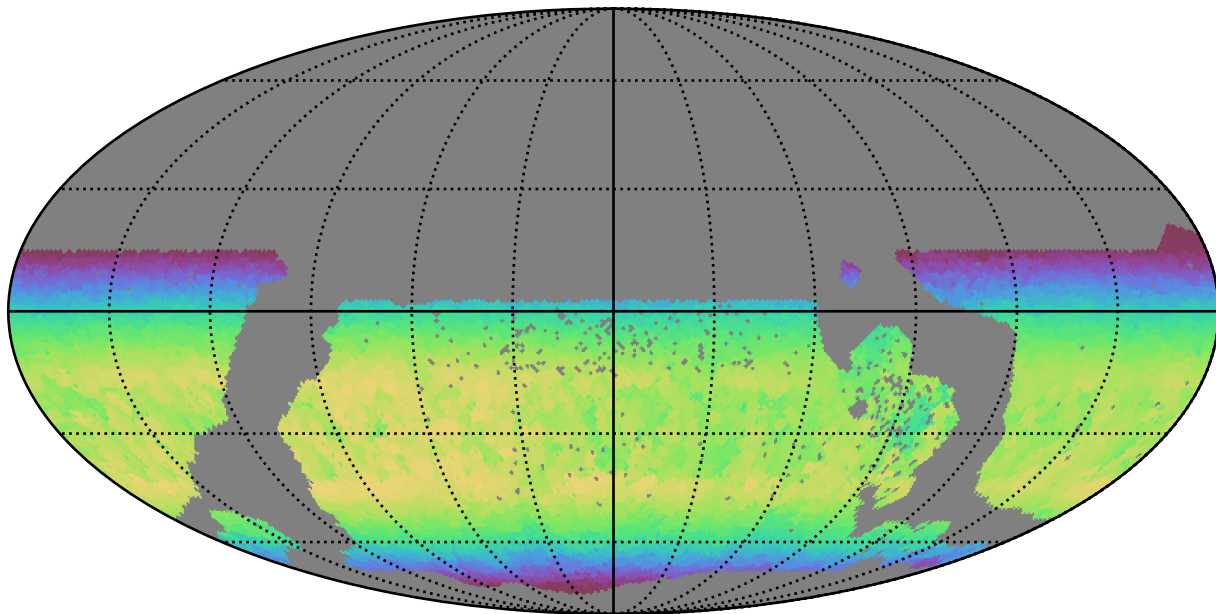
too_100_1v3.4_10yrs WFD y band: Max skyBrightness
