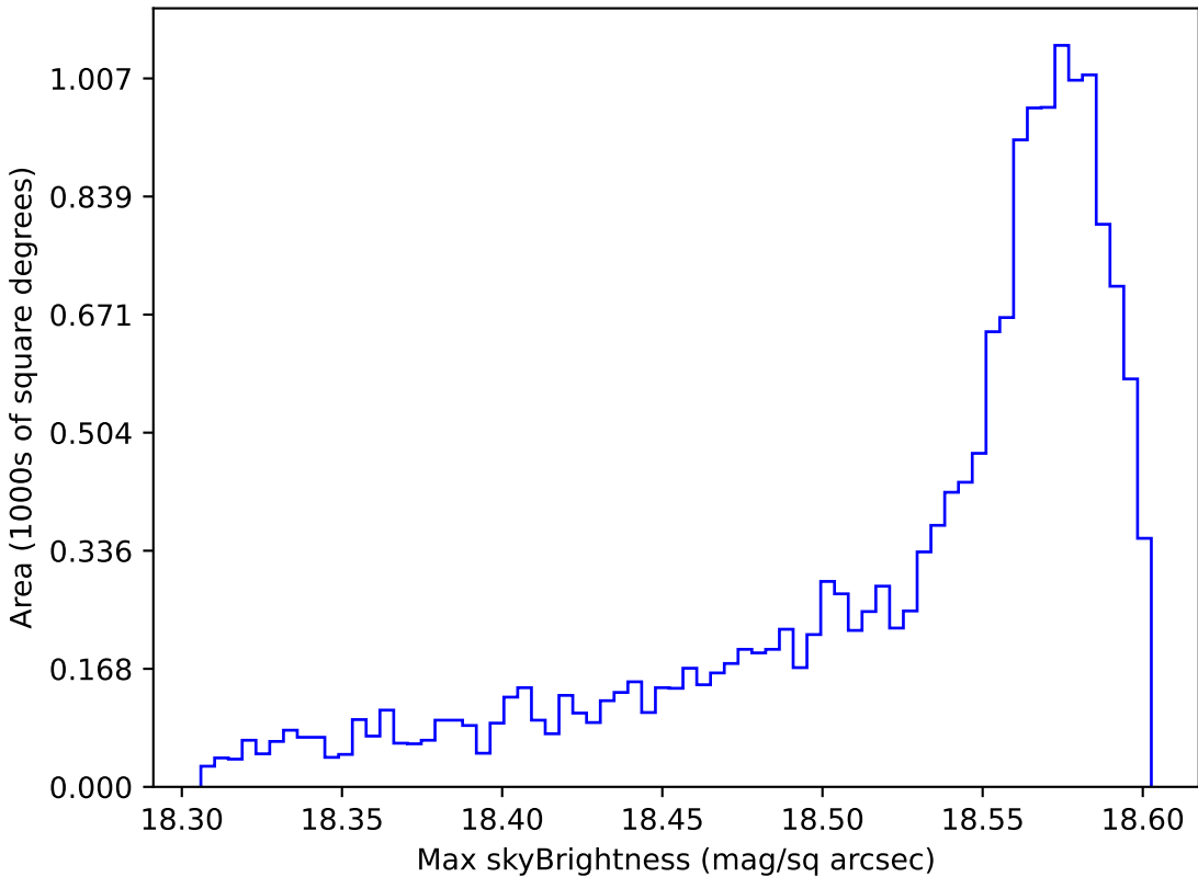
too_100_1v3.4_10yrs WFD y band: Max skyBrightness
