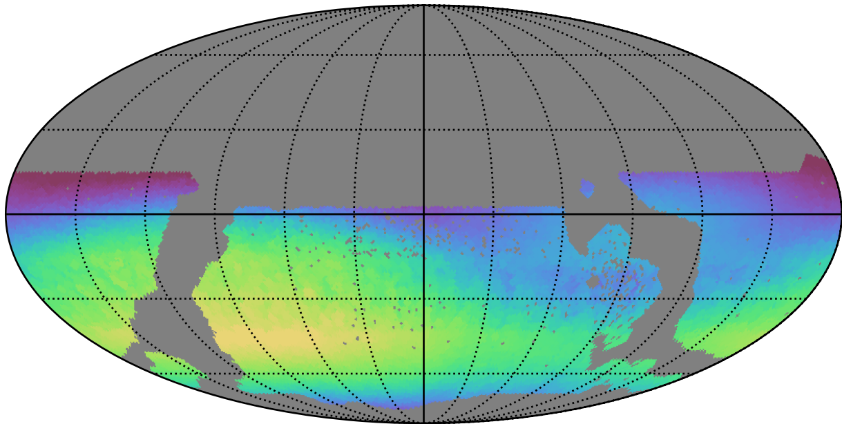
too_100_1v3.4_10yrs WFD u band: Max skyBrightness
