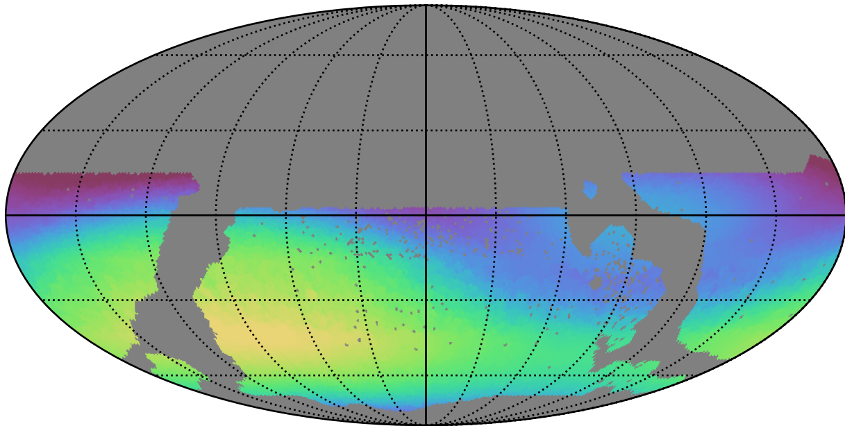
too_100_1v3.4_10yrs WFD r band: Max skyBrightness
