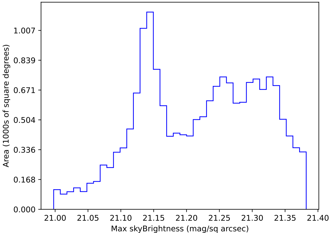
too_100_1v3.4_10yrs WFD r band: Max skyBrightness
