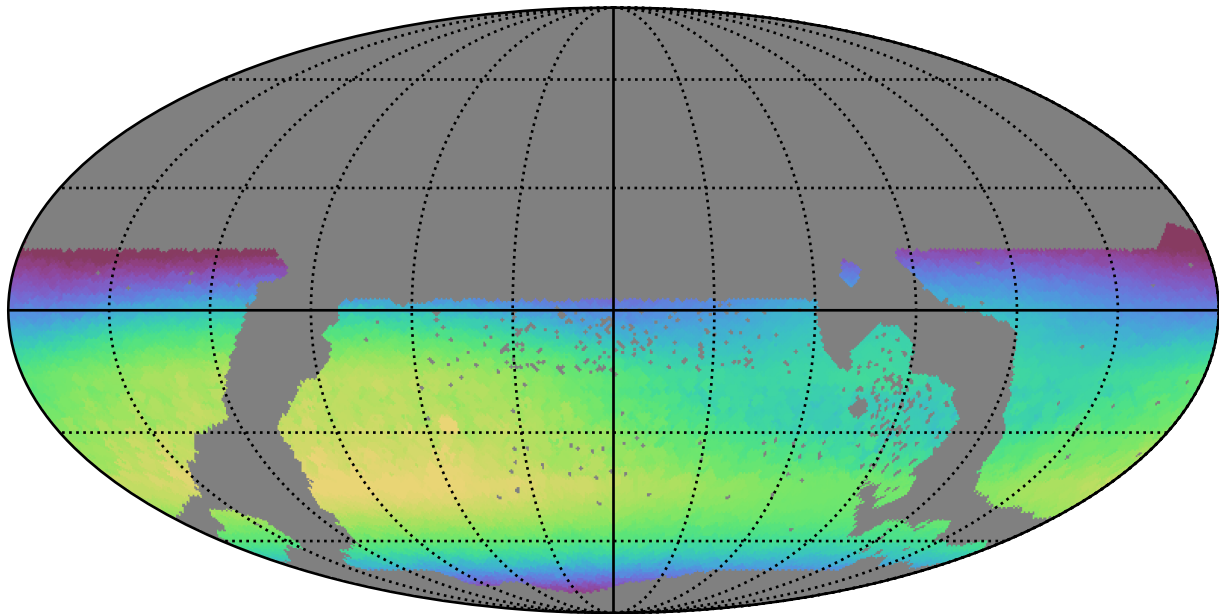
too_100_1v3.4_10yrs WFD i band: Max skyBrightness
