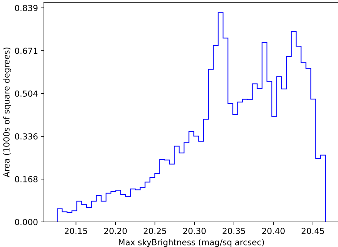
too_100_1v3.4_10yrs WFD i band: Max skyBrightness
