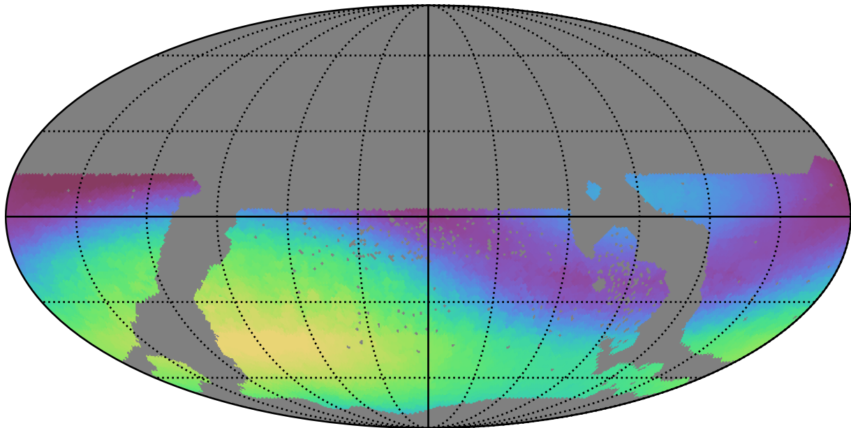
too_100_1v3.4_10yrs WFD g band: Max skyBrightness
