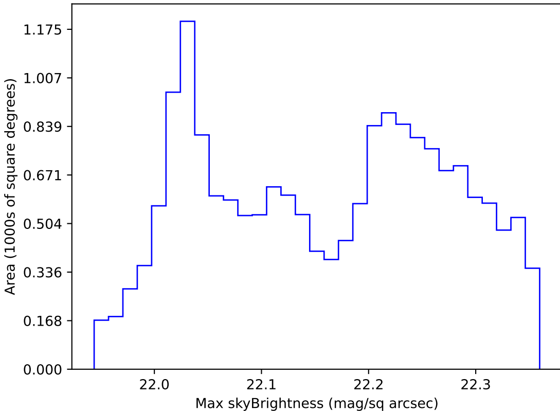
too_100_1v3.4_10yrs WFD g band: Max skyBrightness
