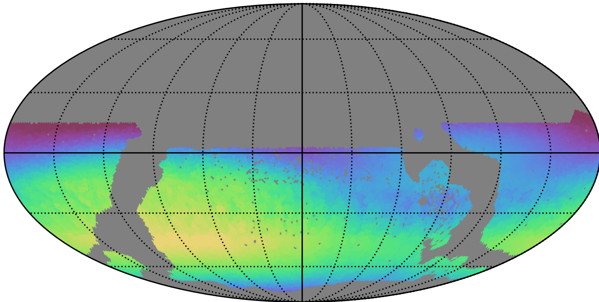
too_100_1v3.4_10yrs WFD all bands: Max skyBrightness
