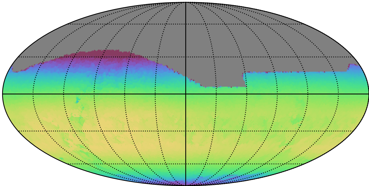
too_100_1v3.4_10yrs All sky z band: Max skyBrightness
